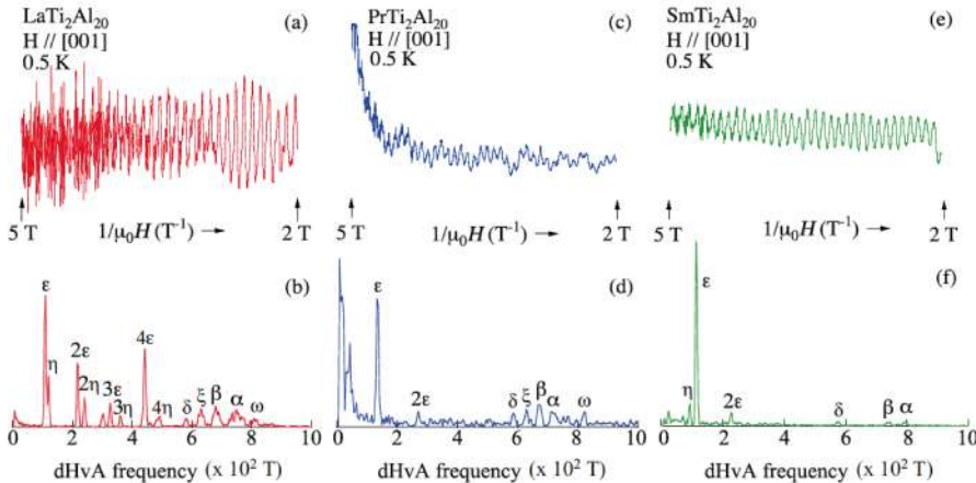
RTi 2 Al 20 (R=La,Pr,Sm)のdHvA効果
